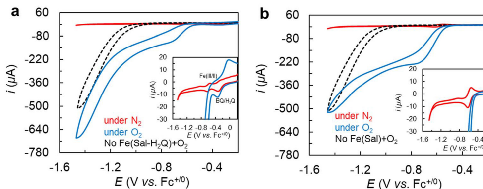
Fig. 1 Cyclic voltammograms of (a) \text{Fe}(\text{Sal-H}_2\text{Q}) and (b) \text{Fe}(\text{Sal}) under \text{N}_2 (red trace) and \text{O}_2 (blue trace). Conditions: 0.5 mM each of (Sal- \text{H}_2\text{Q} ), and \text{Fe}(\text{Sal}) , 300 mM \text{AcOH} , 0.1 M \text{Bu}_4\text{NBF}_4 , acetonitrile. Working electrode: glassy carbon, reference electrode: \text{Ag}/\text{AgCl} , counter electrode: Pt wire, scan rate = 50 \text{ mV s}^{-1} . Grey trace: blank glassy carbon under \text{O}_2 .
